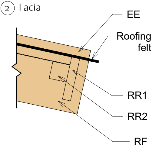
3 Roof Reinforcement
